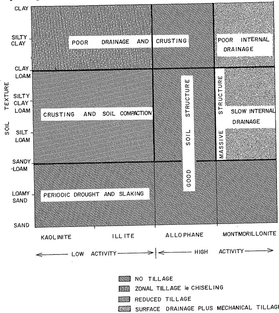
Fig. 3. Tillage systems in the tropics as related to predominant clay minerals, soil texture, and soil management problems (clay mineral activity relates to shrink-swell characteristics).
