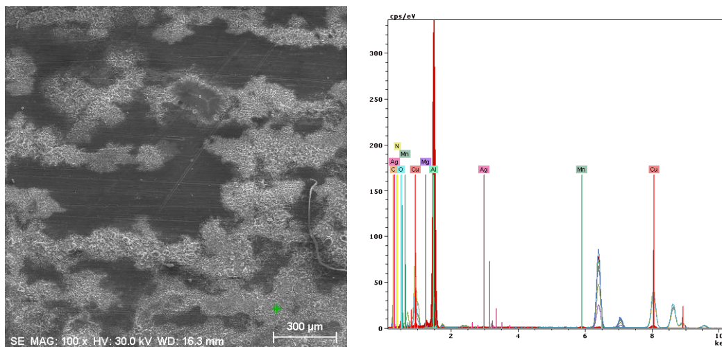
Fig. 4. SEM and EDX analysis of D16 aluminum alloy sample surface
